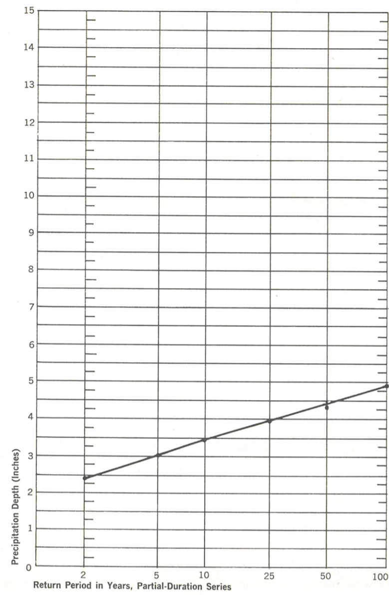
Figure 17. Illustration of use of precipitation-frequency diagrams using values from precipitation-frequency maps and relations at 44°00' N., 115°00' W.
