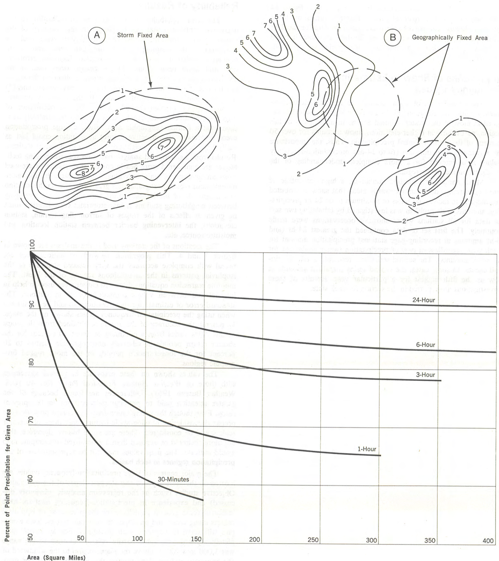
Figure 13. Examples of (A) isohyetal pattern centered over basin as would be the case for storm-centered depth-area curves and (B) two possible occurrences of isohyetal patterns over a geographically fixed area as would be the case in development of curves for a geographically fixed area.
