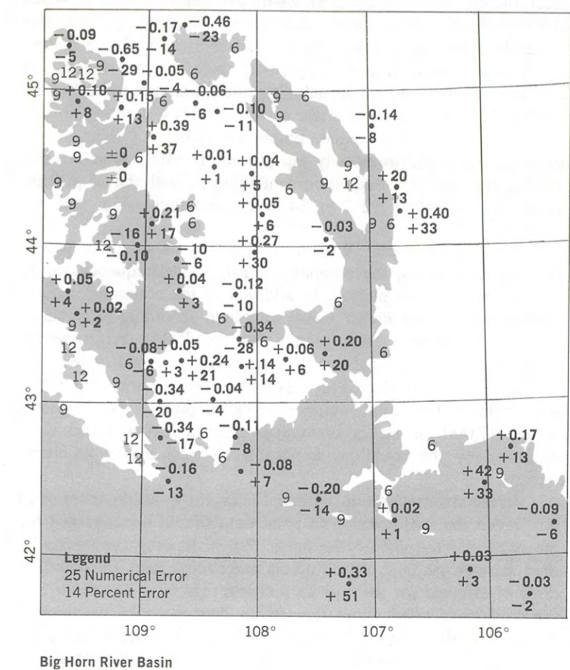
Figure 12. Geographic distribution of errors for equation used to interpolate 2-yr 24-hr precipitation values for the Big Horn River Basin above Saint Xavier, Montana; minor portions of the North Platte, Powder, and Tongue River Basins in eastern Wyoming; and minor portions of the Yellowstone River Basin in northwestern Wyoming and southeastern Montana.
